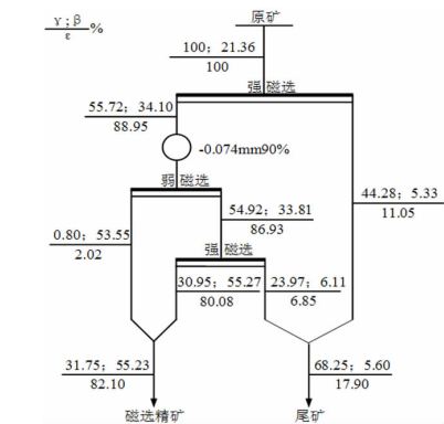
图1 原料制备数质量流程 Fig. 1 Quantity – quality flowsheet of raw material preparation
