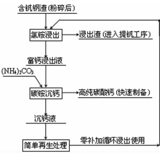
图 1 含钒钢渣中负组元钙净化与回收新工艺 Fig. 1 New process of purification and recovery of negative component calcium from vanadium-bearing steel slag
