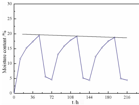
图6 98% RH脱镍硅渣的循环吸放湿曲线 Fig. 6 Cyclic absorption and dehumidification curves of De-nickel silicon slag at 98% RH
