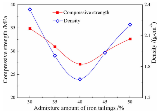
图7 铁尾矿掺入质量分数对微晶泡沫玻璃性能的影响 Fig. 7 Effects of the content of iron tailings on the properties of foam glass - ceramics
