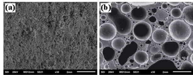
图 2 试样的微观形貌图(a - 微晶玻璃, b - 微晶泡沫玻璃) Fig. 2 SEM images of the test samples (a - basic glass, b - foam glass - ceramics)
