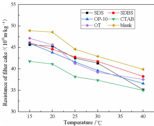
图 9 不同温度对赤铁矿精矿滤饼比阻的影响 Fig. 9 Effects of temperature on the filter cake resistance of hematite concentrate
