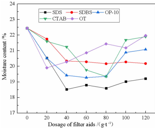
图 4 不同助滤剂用量对赤铁矿精矿含水率的影响 Fig. 4 Effects of filter aids dosages on the filter cake moisture content of hematite concentrate
