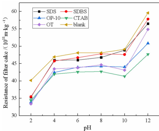
图 7 不同 pH 对赤铁矿精矿滤饼比阻的影响 Fig. 7 Effects of pH on the filter cake resistance of hematite concentrate
