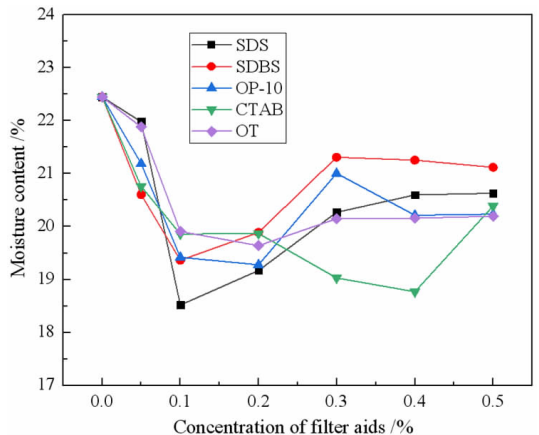
图 6 不同助滤剂浓度对赤铁矿精矿含水率的影响 Fig. 6 Effects of filter aids concentration on the filter cake moisture content of hematite concentrate
