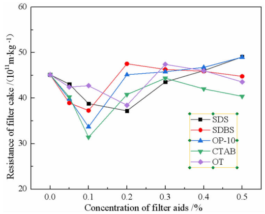
图 5 不同助滤剂浓度对赤铁矿精矿滤饼比阻的影响 Fig. 5 Effects of filter aids concentration on the filter cake resistance of hematite concentrate
