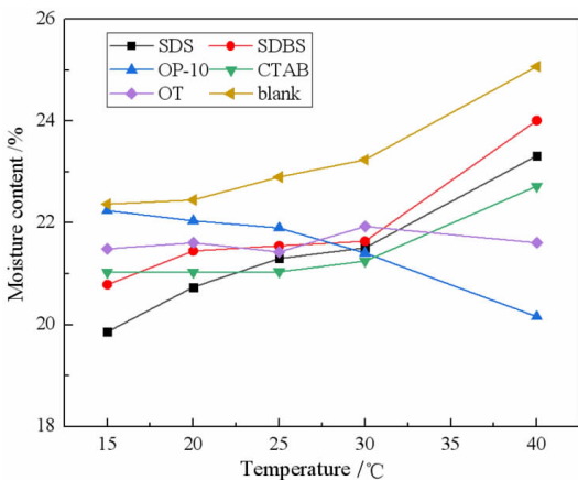
图 10 不同温度对赤铁矿精矿含水率的影响 Fig. 10 Effects of temperature on the filter cake moisture content of hematite concentrate
