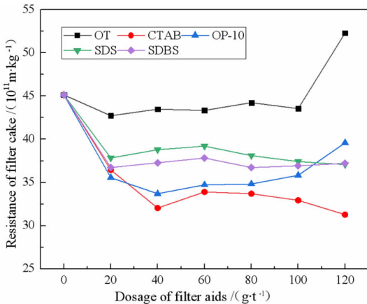
图 3 不同助滤剂用量对赤铁矿精矿滤饼比阻的影响 Fig. 3 Effects of filter aids dosages on the filter cake resistance of hematite concentrate
