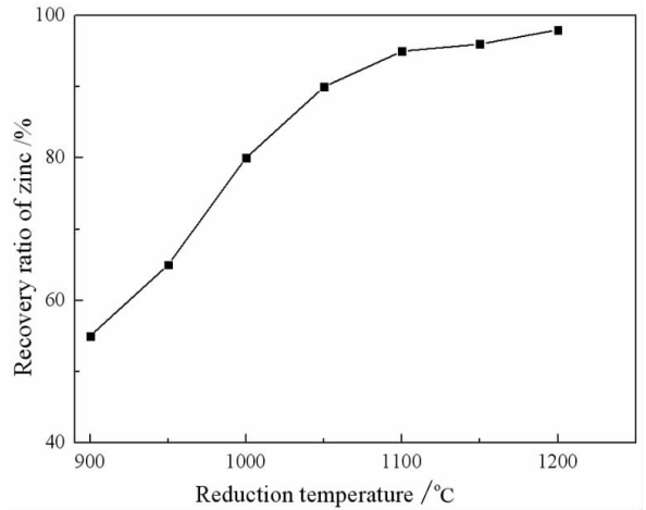
图4 还原温度对锌回收率的影响 Fig. 4 Effect of reduction temperature on the recovery ratio of zinc
