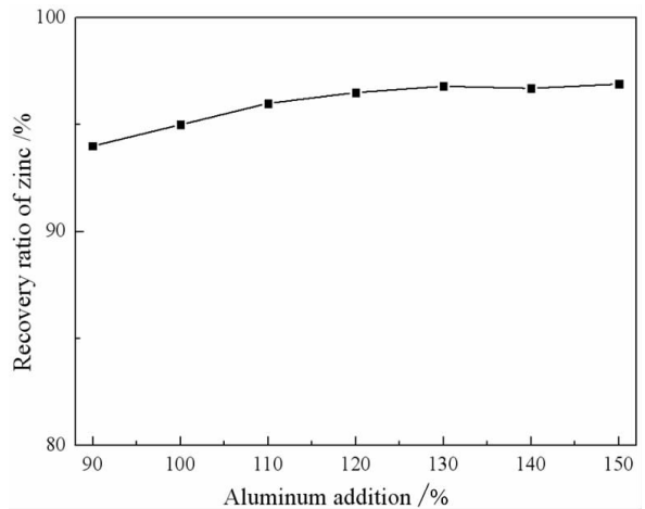
图5 铝粉添加量对锌回收率的影响 Fig. 5 Effect of the dosage of aluminum on the recovery ratio of zinc
