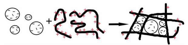
图 5 网捕卷扫机理示意图 Fig. 5 Schematic diagram of the mechanism of net catching and sweeping
