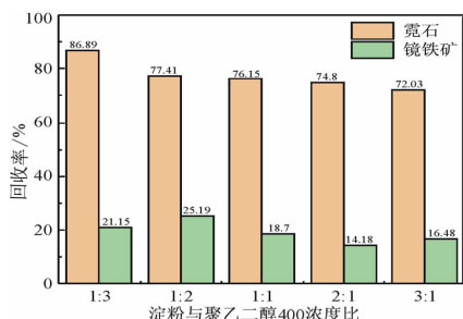
图 7 不同混合比例淀粉和聚乙二醇 400 对镜铁矿及霓石的抑制效果 Fig. 7 Effect of mixing ratio of starch and PEG 400 on specularite and aegirite
