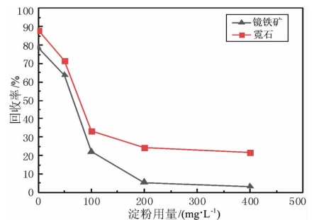
图 6 淀粉浓度对镜铁矿及霓石的抑制效果 Fig. 6 Effect of starch concentration on the floatability of specularite and aegirite
