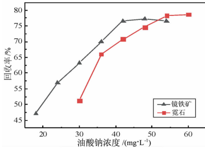
图 3 油酸钠浓度对霓石和镜铁矿可浮性的影响 Fig. 3 Effect of sodium oleate concentration on the floatability of aegirite and specularite
