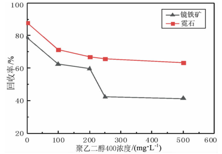
图 5 聚乙二醇 400 浓度对镜铁矿和霓石可浮性的影响 Fig. 5 Effect of PEG 400 concentration on the floatability of specularite and aegirite
