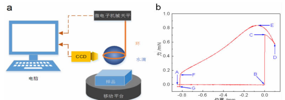
图 2 a, 试验系统; b, 典型的水滴在矿物表面的黏附力曲线 Fig. 2 Experimental system(a); A typical force curve for a water droplet on mineral surface(b)
