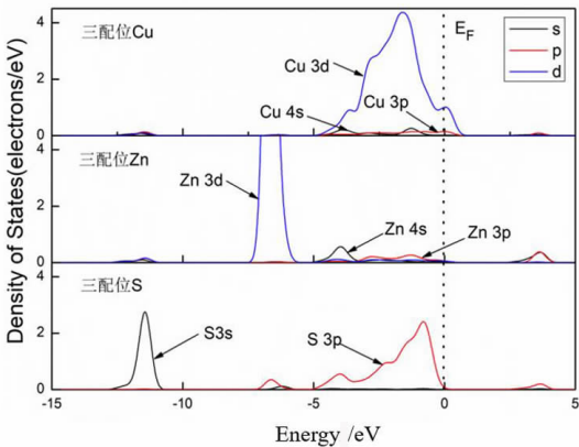
图4 铜活化闪锌矿表面原子态密度 Fig. 4 The atomic partial points density of states of the surface of copper – activated sphalerite
