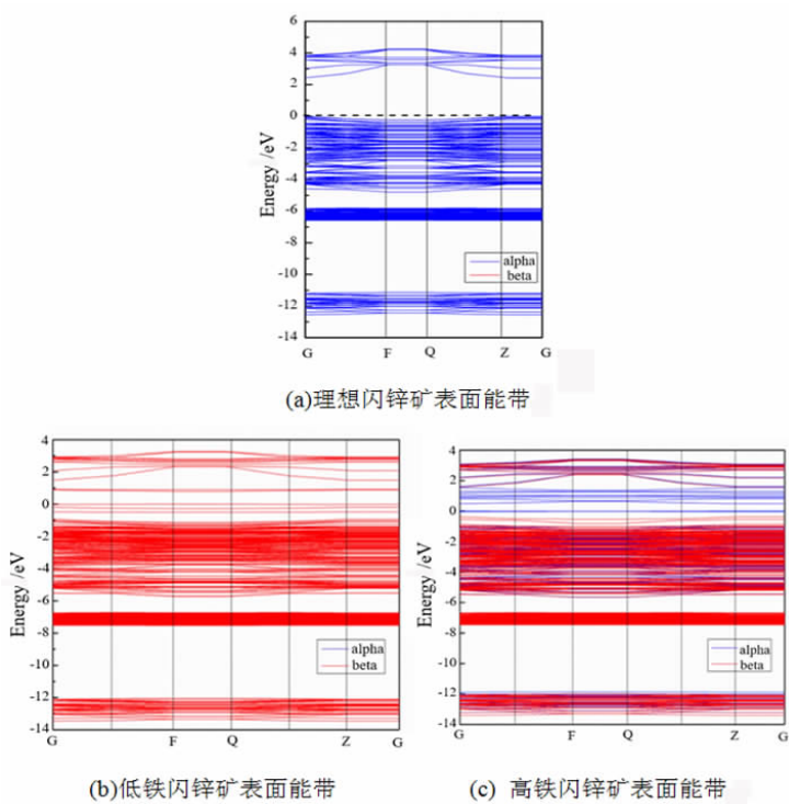
图3 不同含铁量的闪锌矿表面能带 Fig. 3 Band structure of iron – bearing sphalerite surface: (a) Ideal sphalerite, (b) low iron and (c) high iron
