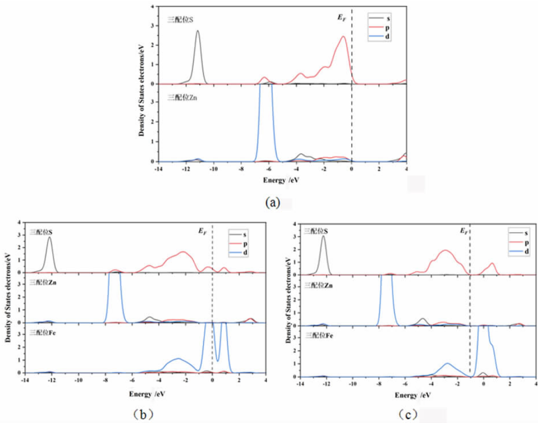
图 2 不同铁含量的闪锌矿表面态密度:(a)理想闪锌矿表面态密度 (b)高铁闪锌矿表面态密度 (c)高铁闪锌矿表面态密度 Fig. 2 The atomic partial density of states of the surface of iron – bearing sphalerite:(a) Ideal sphalerite, (b) low iron and (c) high iron
