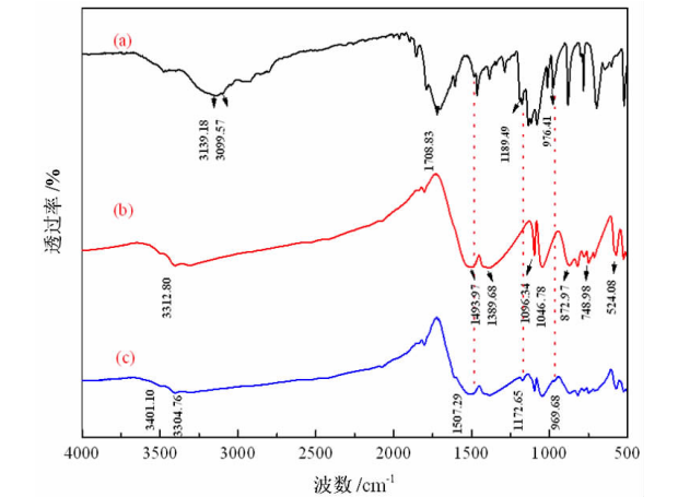
图 10 邻苯二羟肟酸处理前后孔雀石的红外光谱图 Fig. 10 Infrared spectrum of malachite before and after treatment with phthalic acid
