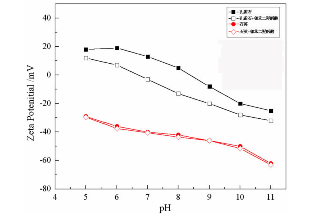
图 9 邻苯二羟肟酸捕收剂处理前后孔雀石和石英的 Zeta 电位与 pH 关系图 Fig. 9 Relationship between zeta potential and pH of malachite and quartz before and after treatment with phthalic acid
