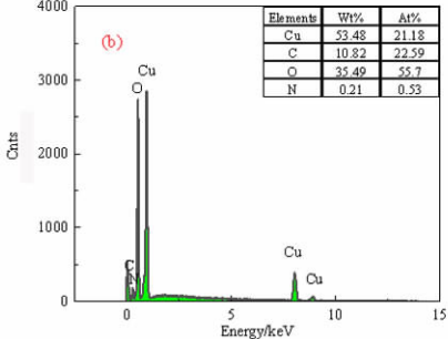
(a)孔雀石的EDS;(b)孔雀石+邻苯二羟膦酸的EDS 图8 邻苯二羟膦酸处理前后孔雀石的SEM-EDS谱图 (a)EDS of malachite;(b)EDS of malachite with o-phenylhydroxamic acid Fig. 8 SEM-EDS spectrum of malachite before and after treatment with phthalic acid
