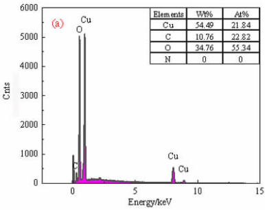
(a)孔雀石的EDS;(b)孔雀石+邻苯二羟膦酸的EDS 图8 邻苯二羟膦酸处理前后孔雀石的SEM-EDS谱图 (a)EDS of malachite;(b)EDS of malachite with o-phenylhydroxamic acid Fig. 8 SEM-EDS spectrum of malachite before and after treatment with phthalic acid
