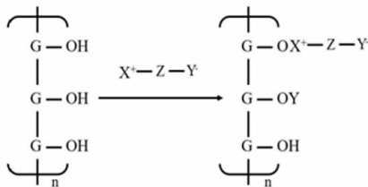
(注: X—阳离子化试剂; Y—阴离子化试剂; X—Z—Y 两亲离子) 图 4 两亲离子与淀粉反应示意图 Fig. 4 Schematic diagram of the reaction between amphiphilic ions and starch
