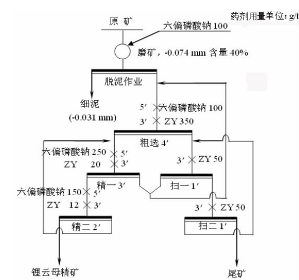
图 5 锂云母浮选闭路试验流程 Fig. 5 Flowsheet of lithium mica flotation closed - circuit tests
