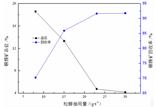
图 7 松醇油用量对铜浮选指标的影响 Fig. 7 The effect of terpene oil dosage on copper flotation index
