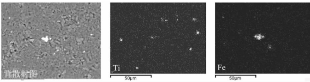
图 3 −0.010 mm 粒级背散射图及 Ti、Fe 元素面扫描图 Fig. 3 Backscattering diagram of −0.010 mm classes of kaolin and scanning diagram of Ti and Fe elements
