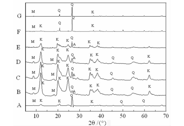
(K:高岭石;Q:石英;M:白云母;A:钠长石) A:原矿;B: -0.002 mm; C: -0.005 + 0.002 mm; D: -0.010 + 0.005 mm; E: -0.020 + 0.010 mm; F: -0.030 + 0.020 mm; G: -0.045 + 0.030 mm
