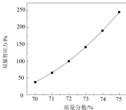
图 11 屈服剪切应力拟合曲线 Fig. 11 Fitting curve of yield-shear stress
