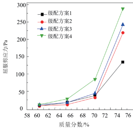
图 1 质量分数对屈服剪切应力的影响 Fig. 1 Effect of mass fraction on yield-shear stress
