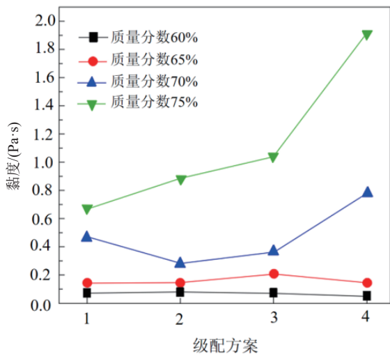
图 4 粒径级配对塑性黏度的影响 Fig. 4 Effect of particle size grading distribution on plastic viscosity
