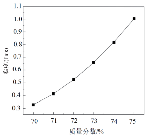
图 12 塑性黏度拟合曲线 Fig. 12 Fitting curve of plastic viscosity
