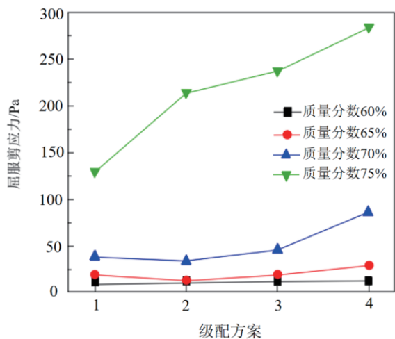
图 3 粒径级配对屈服剪切应力的影响 Fig. 3 Effect of particle size grading distribution on yield-shear stress
