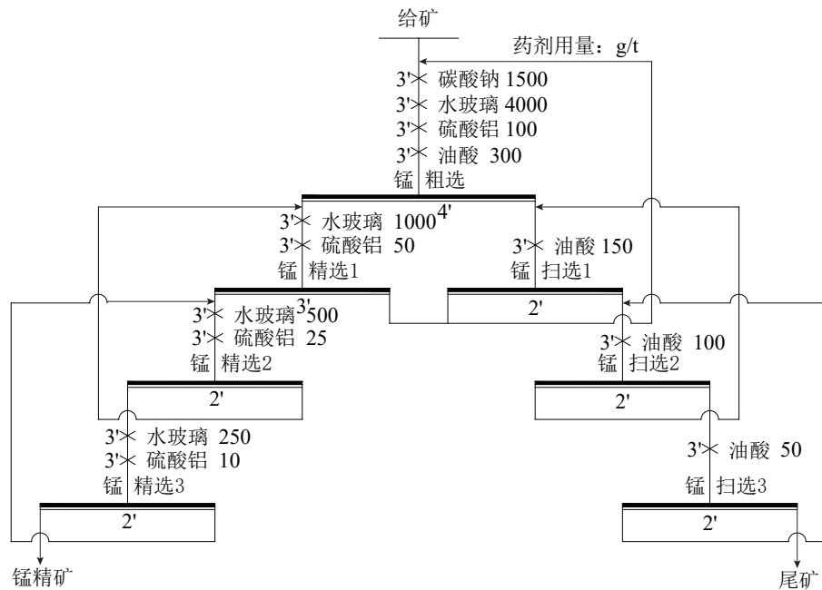
图 6 浮选闭路实验流程 Fig. 6 Experimental flowsheet of the closed-circuit flotation
