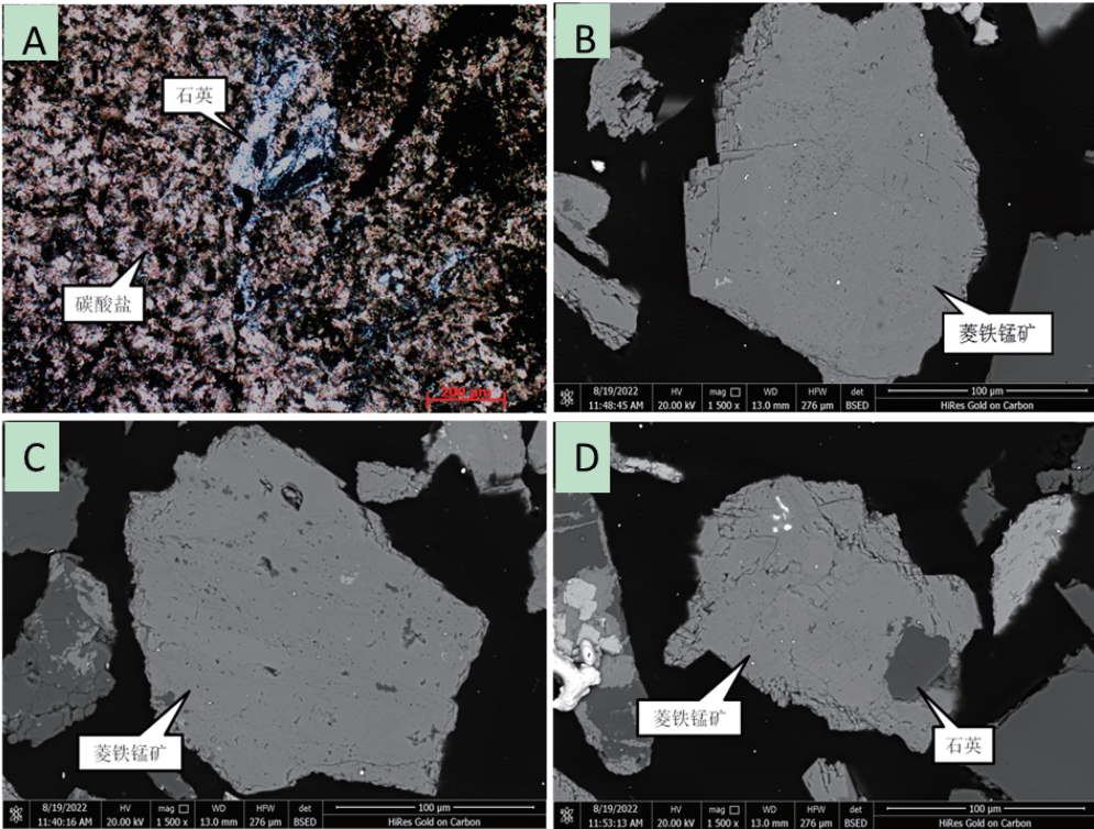
A—细粒碳酸盐矿物; B—菱铁锰矿集合体; C—单体解离菱铁锰矿; D—菱铁锰矿连体 图 1 MLA 分析结果 A. Fine carbonates; B. Aggregation of ferrohodochochroite; C. Dissociated ferrohodochochroite; D. Connection of ferrohodochochroite Fig. 1 Analysis results of MLA
